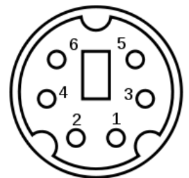
Front view of miniDIN6 male connector
