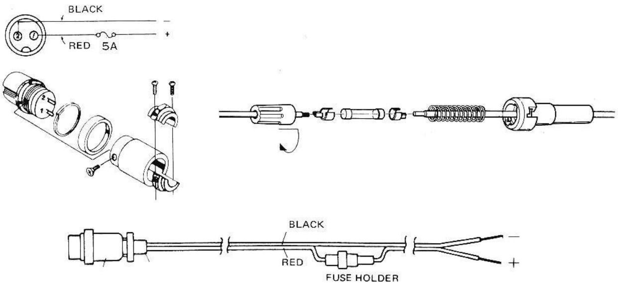
POWER CORD CONNECTIONS
