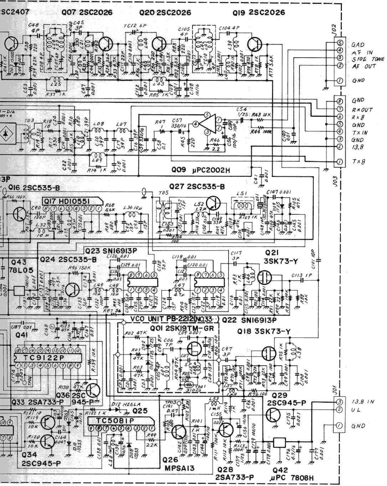
FT-780R(A) PLL UNIT CIRCUIT DIAGRAM
