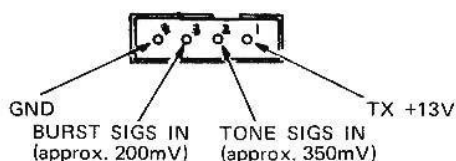
TONE IN CONNECTOR
