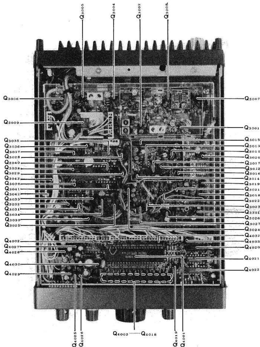
PART LOCATIONS (Top View)
