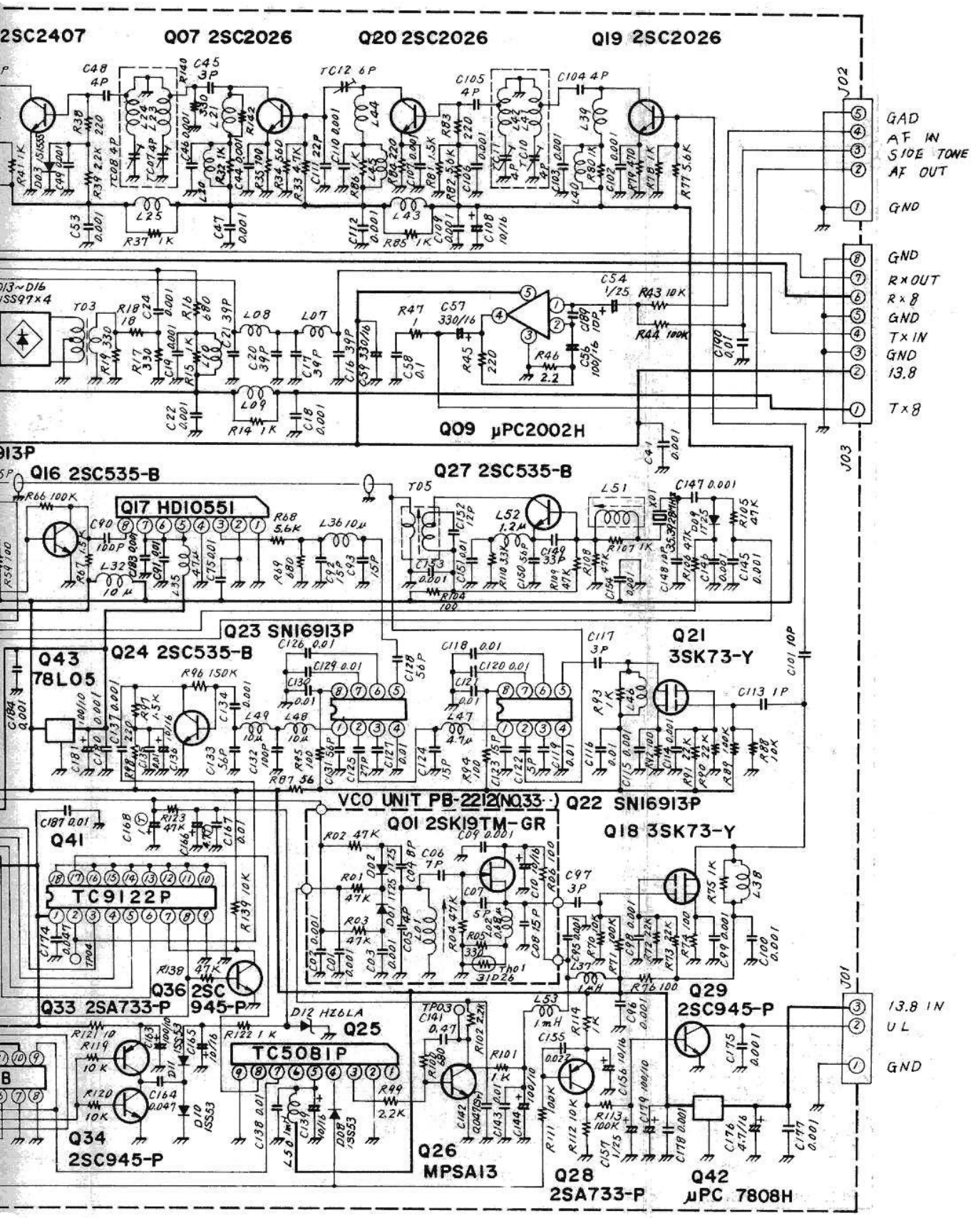
FT-780R(BX) PLL UNIT CIRCUIT DIAGRAM
