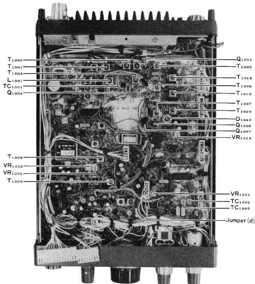
ALIGNMENT AND TEST POINTS FOR RECEIVER
