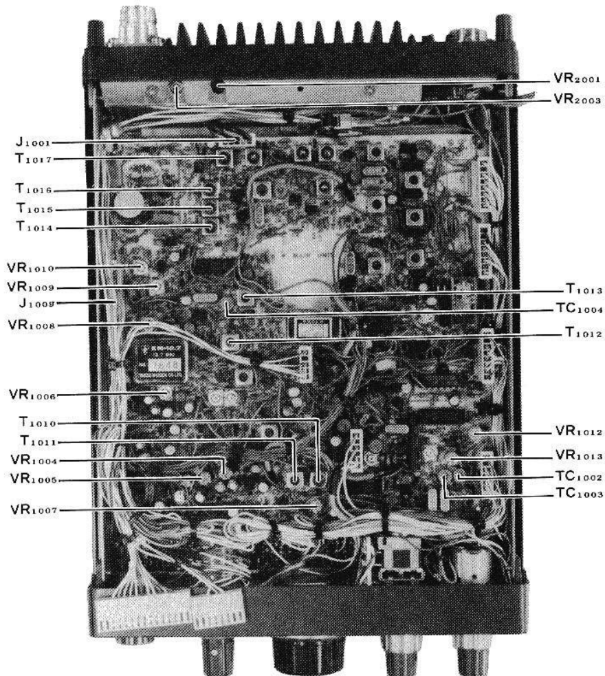
ALIGNMENT AND TEST POINTS FOR TRANSMITTER
