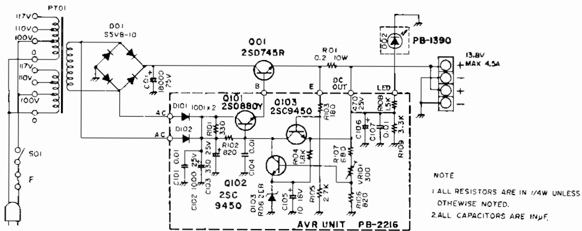
FP-80A POWER SUPPLY
